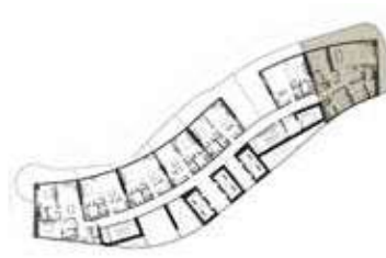
SKY GARDEN 2 BALCONY TYPE 0 TOWER C: LEVEL: 13
