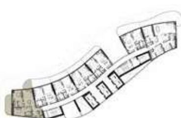
SKY GARDEN 2 BALCONY TYPE 1 TOWER C: LEVEL: 14
